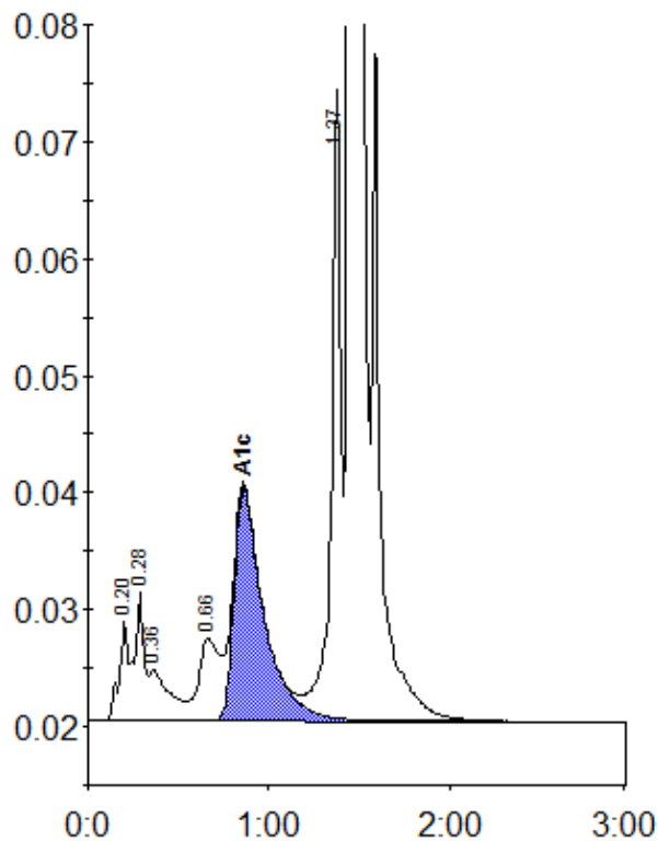
Peak table - ID: 10352152
